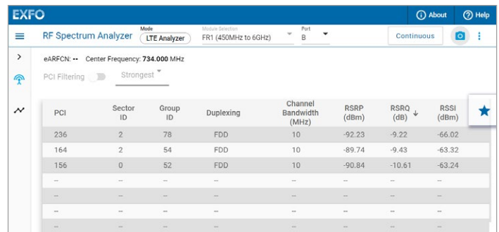
Figure 8. LTE analysis.
